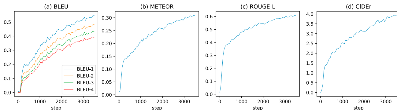
Fig. 7. BLEU-1, -2, -3, -4, METEOR, ROUGE-L, and CIDEr scores on the MICD validation dataset along 3500 training steps (100 training epochs).
