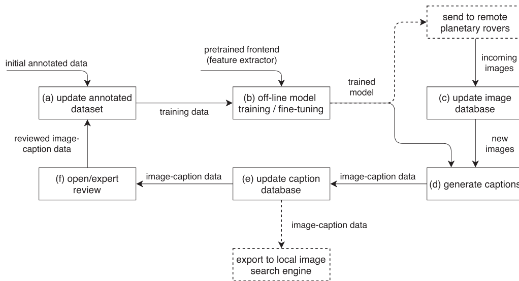
Fig. 2. Workflow of the data aggregation and model retraining pipeline.
