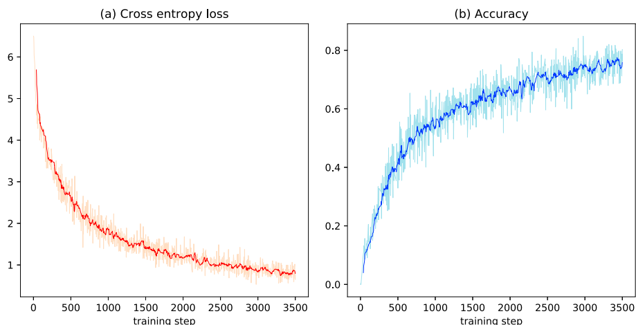
Fig. 6. Learning curves of SCOTI network on MICD training dataset throughout the 3500 training steps (100 training epochs). The highlighted curves are smoothed by averaging 10 nearby sample points from the actual learning curves shown on the background.
