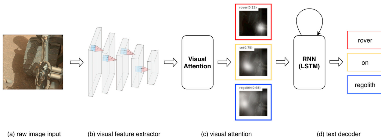
Fig. 1. An illustration on the architecture of SCOTI.
